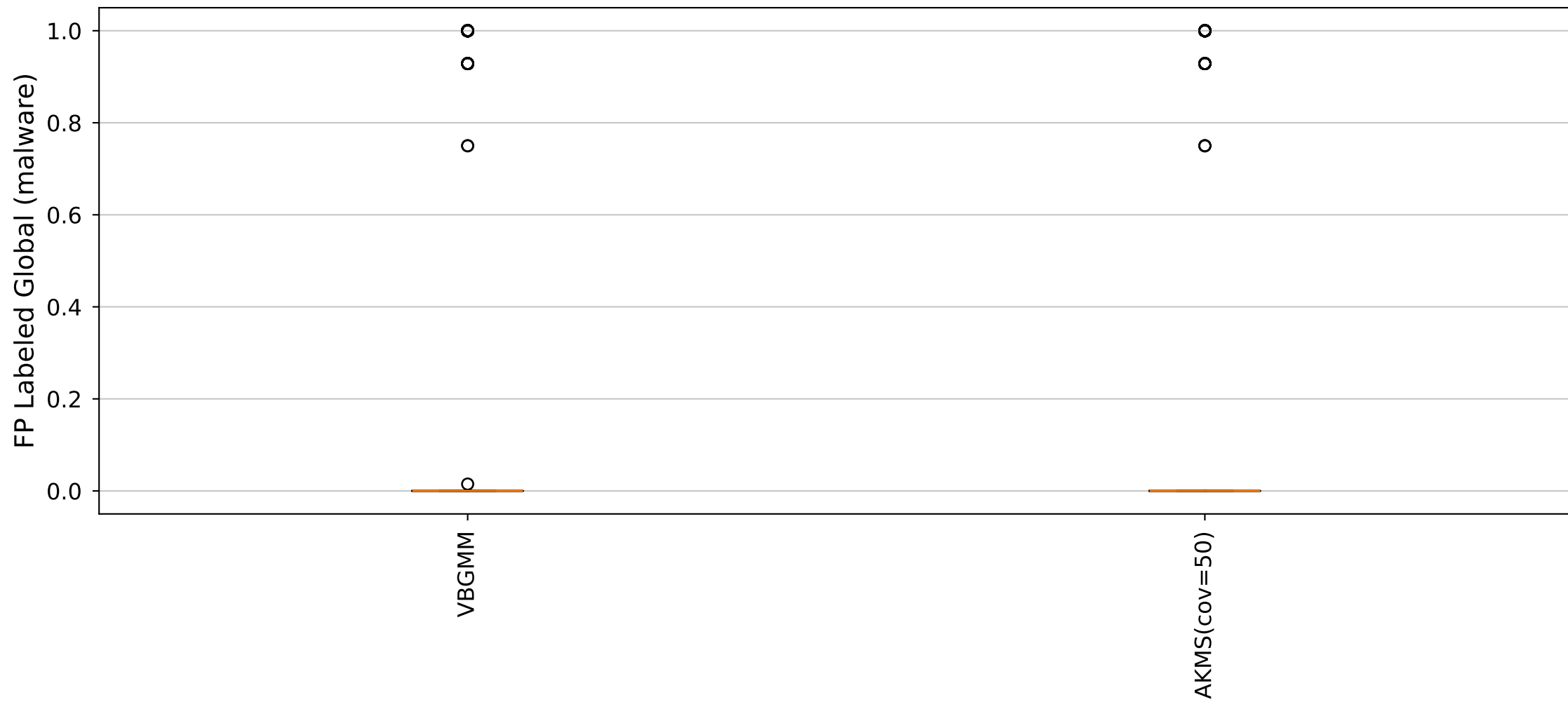
YARA Rules FP Labeled Global (malware) Distribution (Cluster2_Size100 dataset)
